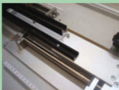
Scale for positioning holes punching on profiles and fabrics.
